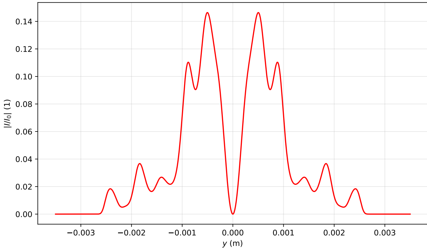
Intensity profile I(x=0, y, z=3.105)/I_0 , P_{in}=9.0P_{cr} , artificial time
